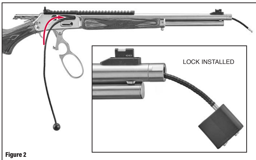
Figure 2 Correct installation of the lock on a Marlin® Model 1895 rifle.
